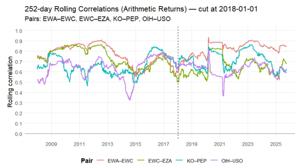
Figure 2. 252-day rolling correlations
